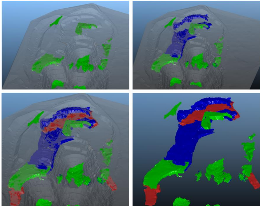
Pictured: The Northern Area. Work done in Phase 6 Pit outline, during Q3. The green sections represent the area mined in January 2025, blue in February and red in March.
