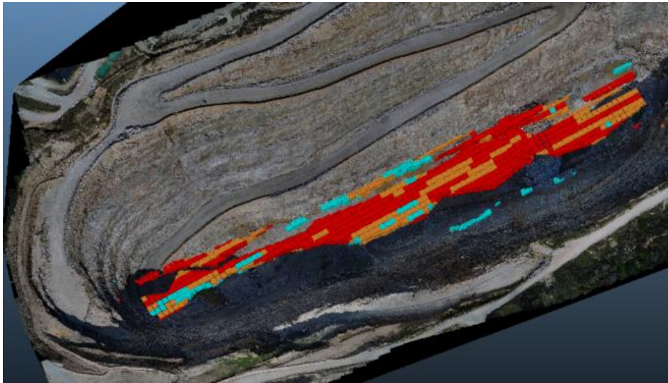
Picture above: The ore production zone during Q3 FY2025 in the Southern Area as per Resource Block Model. Colours represent the grade of the ore. Red for high grade (>0.15% WO 3 ). Orange for lower grade (0.07-0.15% WO 3 ). Blue for very low grade. (0.055-0.07% WO 3 ).
