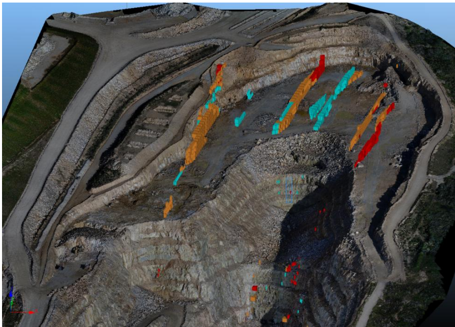
Picture above: The Northern Area as of 31st March 2025. Resources Block Model in Phase 6 Pit outline showing ore block already extracted. Colours represent the grade of the ore. Red for high grade (>0.15% WO 3 ). Orange for lower grade (0.07-0.15% WO 3 ). Blue for very low grade. (0.055-0.07% WO 3 ).
