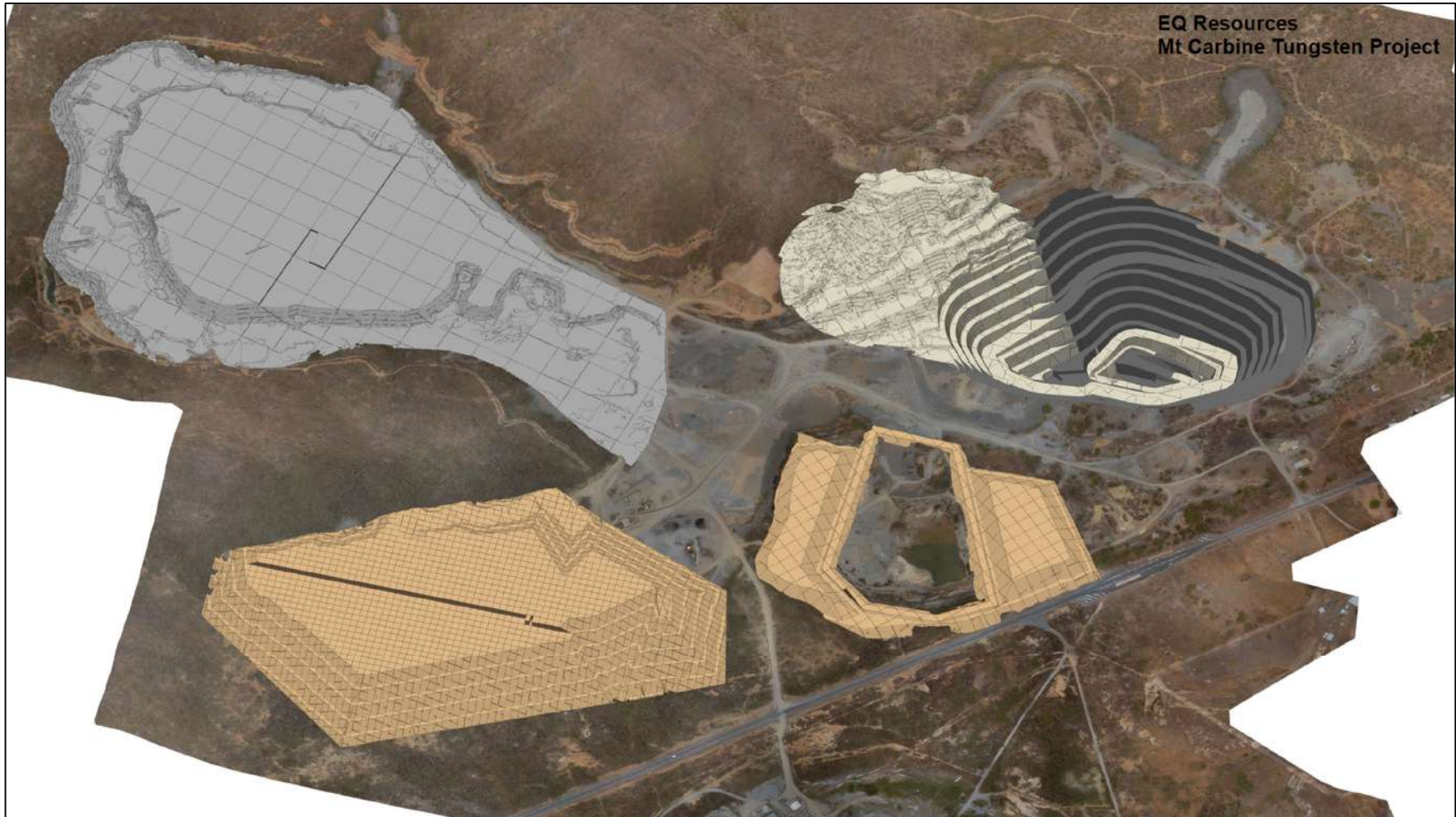
Figure 3-21 - Mine Status at end of 2027
