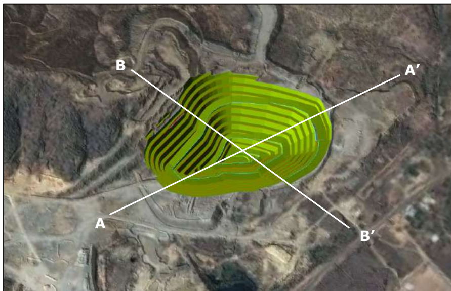
Figure 3-5 – Economic Pit Shell for Mt Carbine
