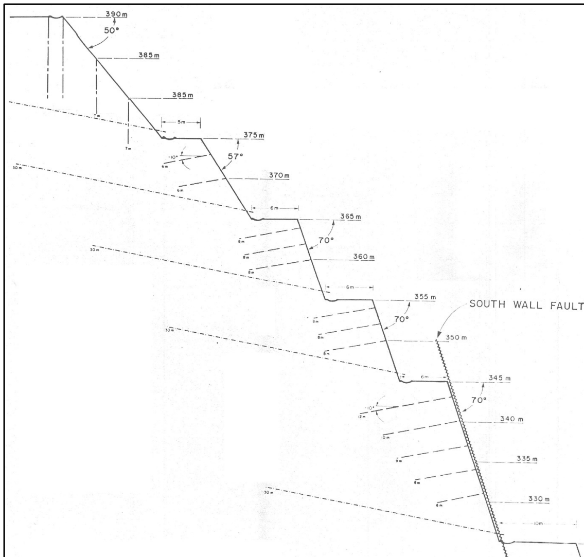
Figure 3-3 –South Wall Geotechnical Design
