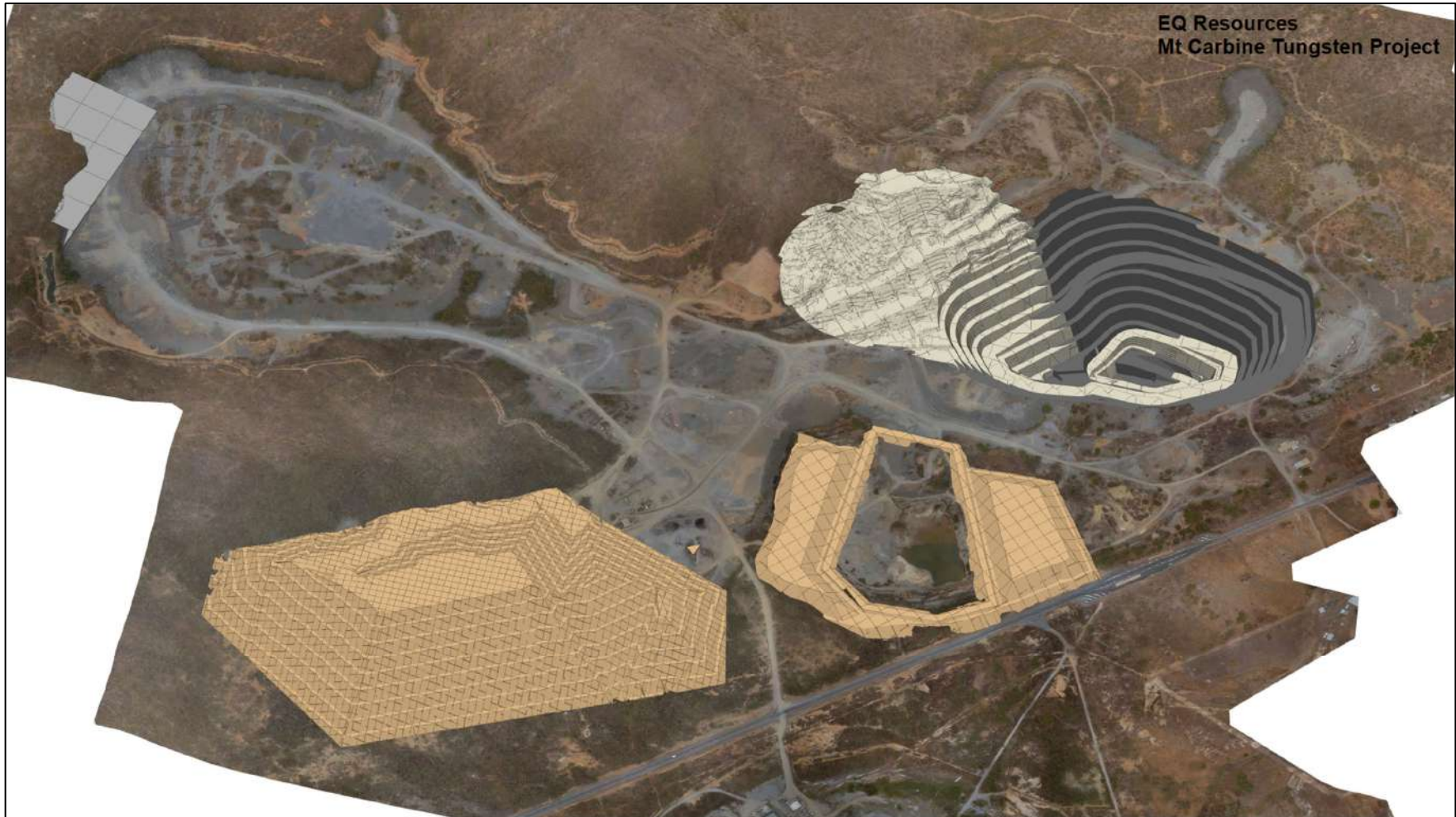
Figure 3-22 – Mine Status at the end of 2036
