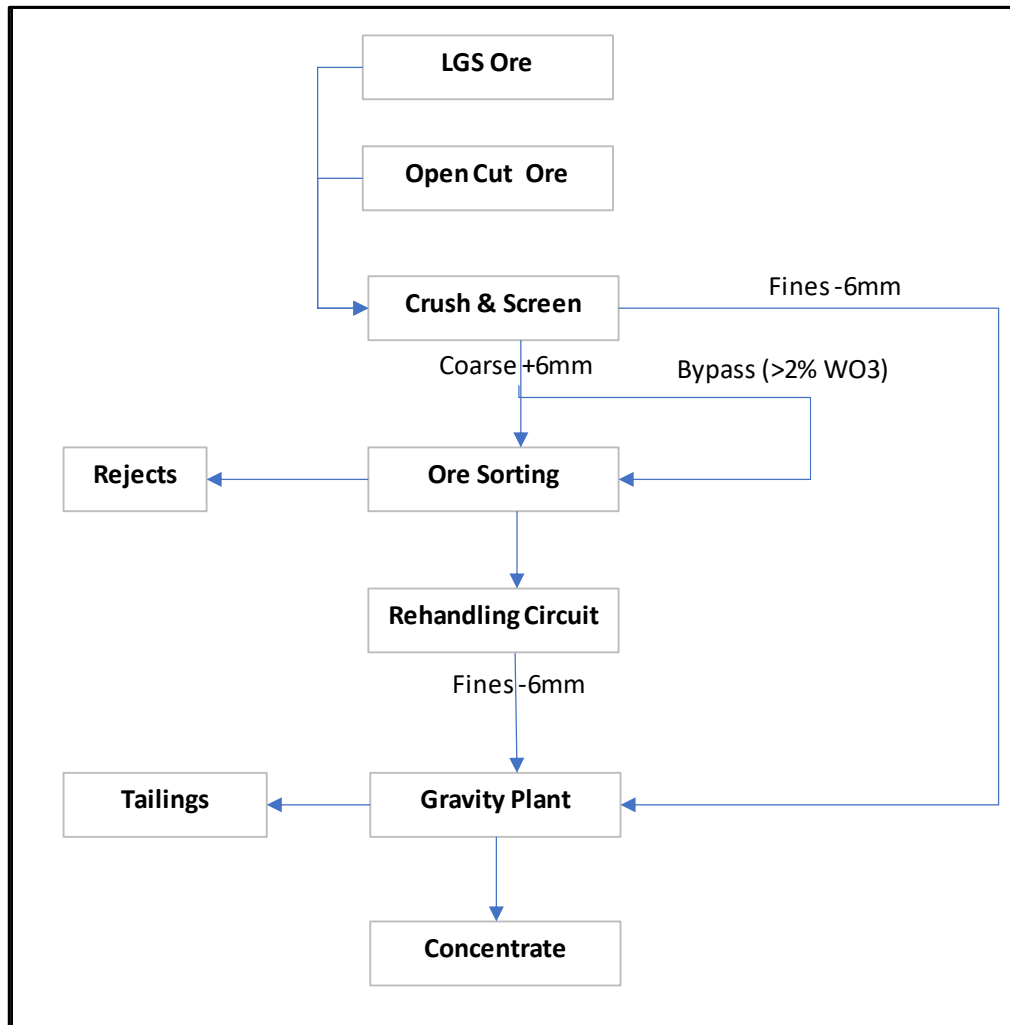
Figure 3-10 – Mt Carbine Ore Processing Flowchart
