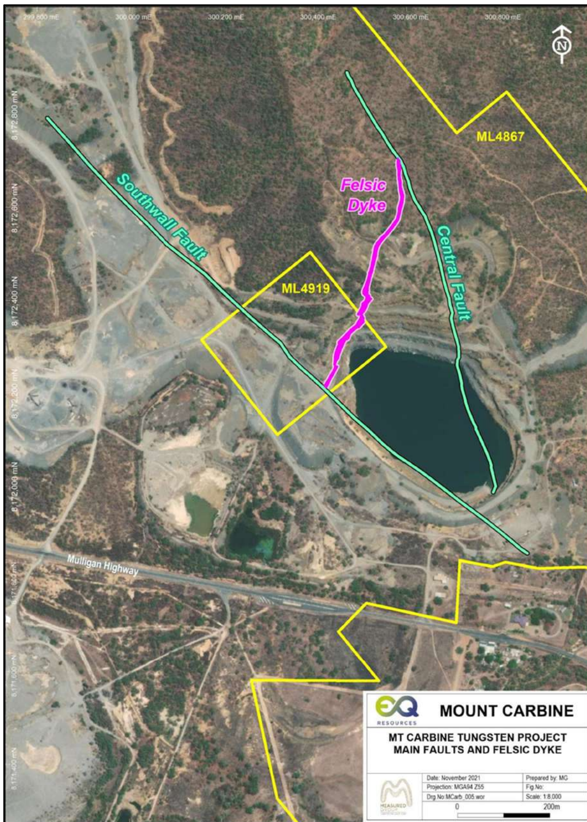
Figure 1-7: Mt Carbine Open Pit Structure
