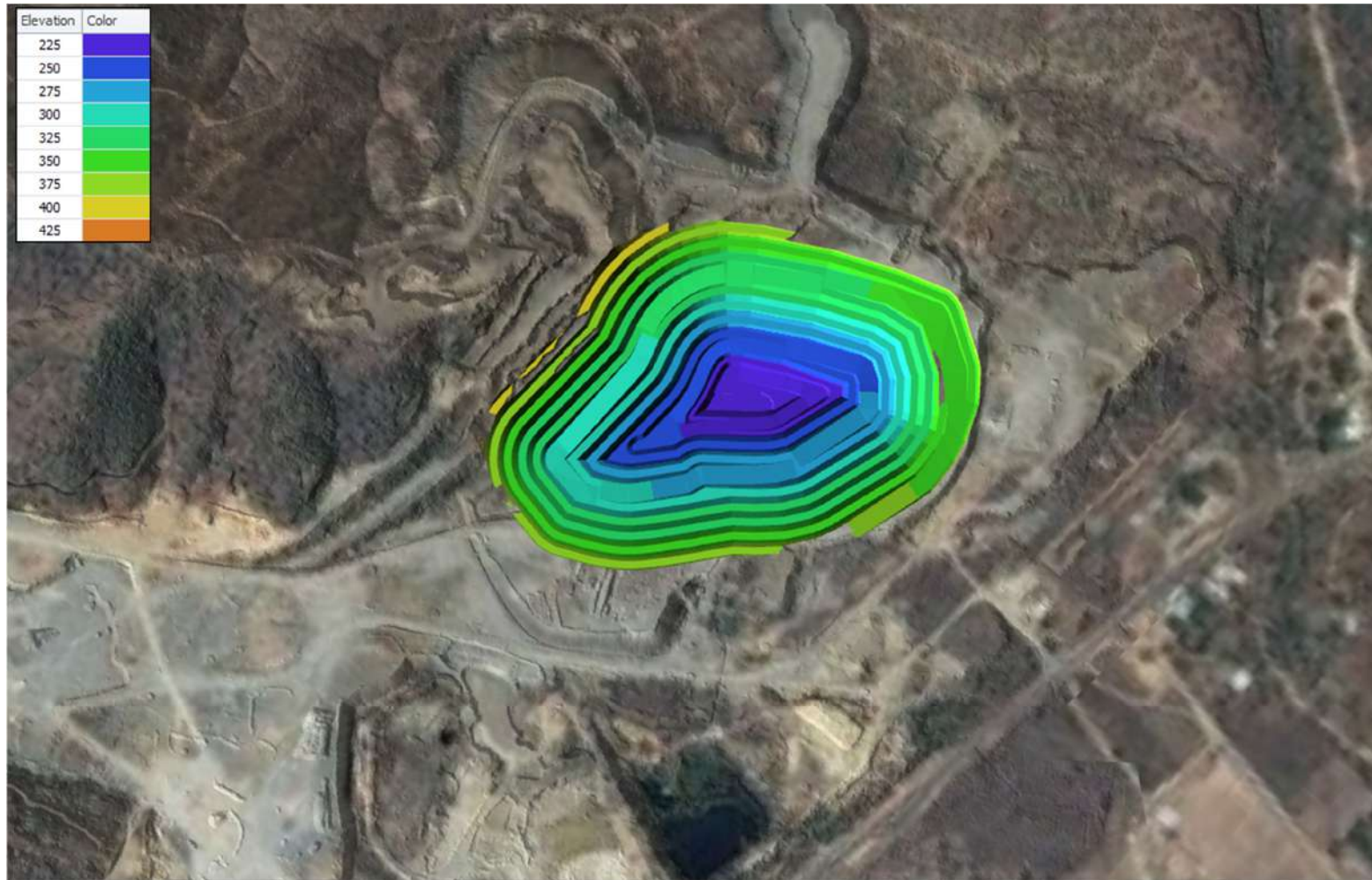
Figure 5-1 – Open Pit Ore Reserve Limits
