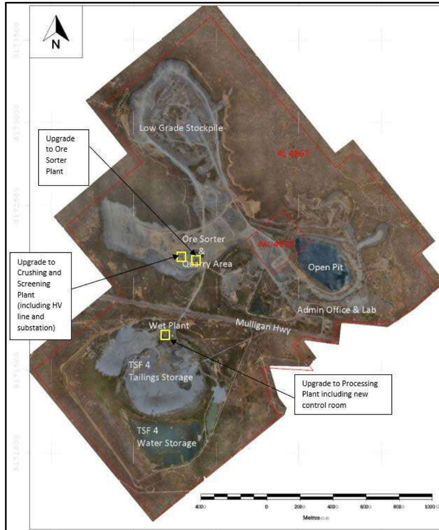
Figure 1-5: Mt Carbine Upgrade Plan
